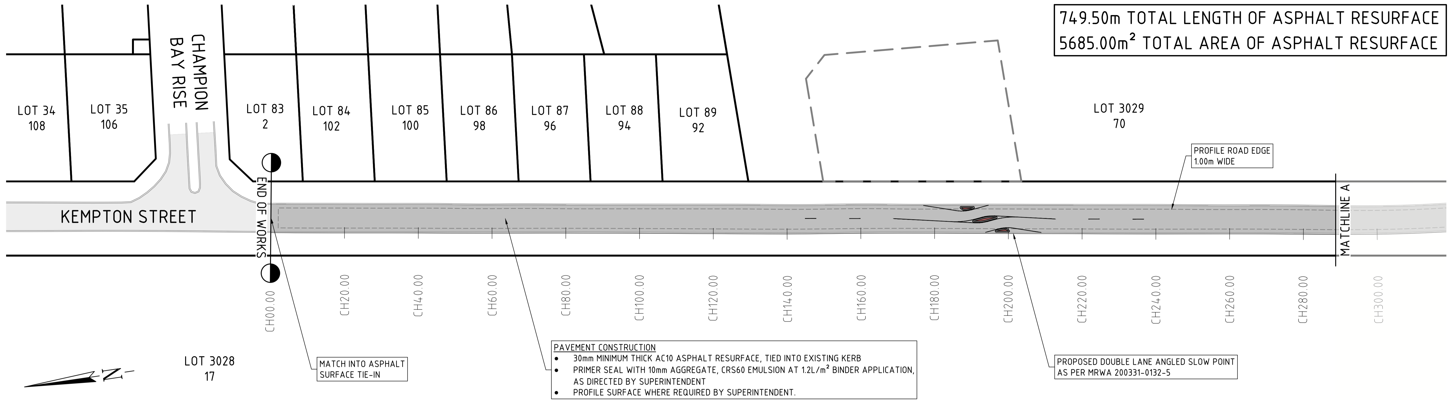
PLAN VIEW - SECTION A SCALE 1:500 @ A1
