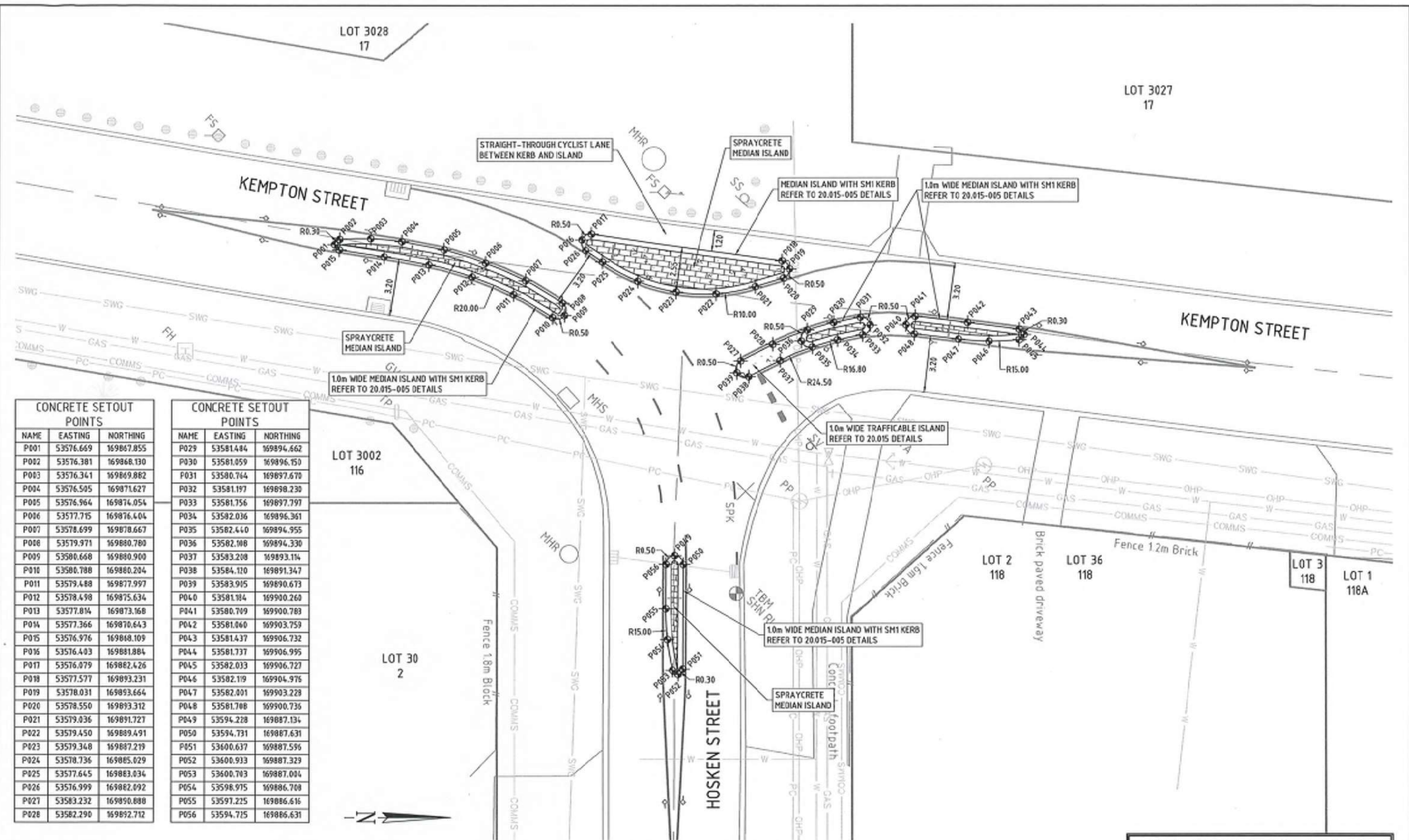
PLAN VIEW - OVERALL PLAN SCALE 1:100 @ A1
