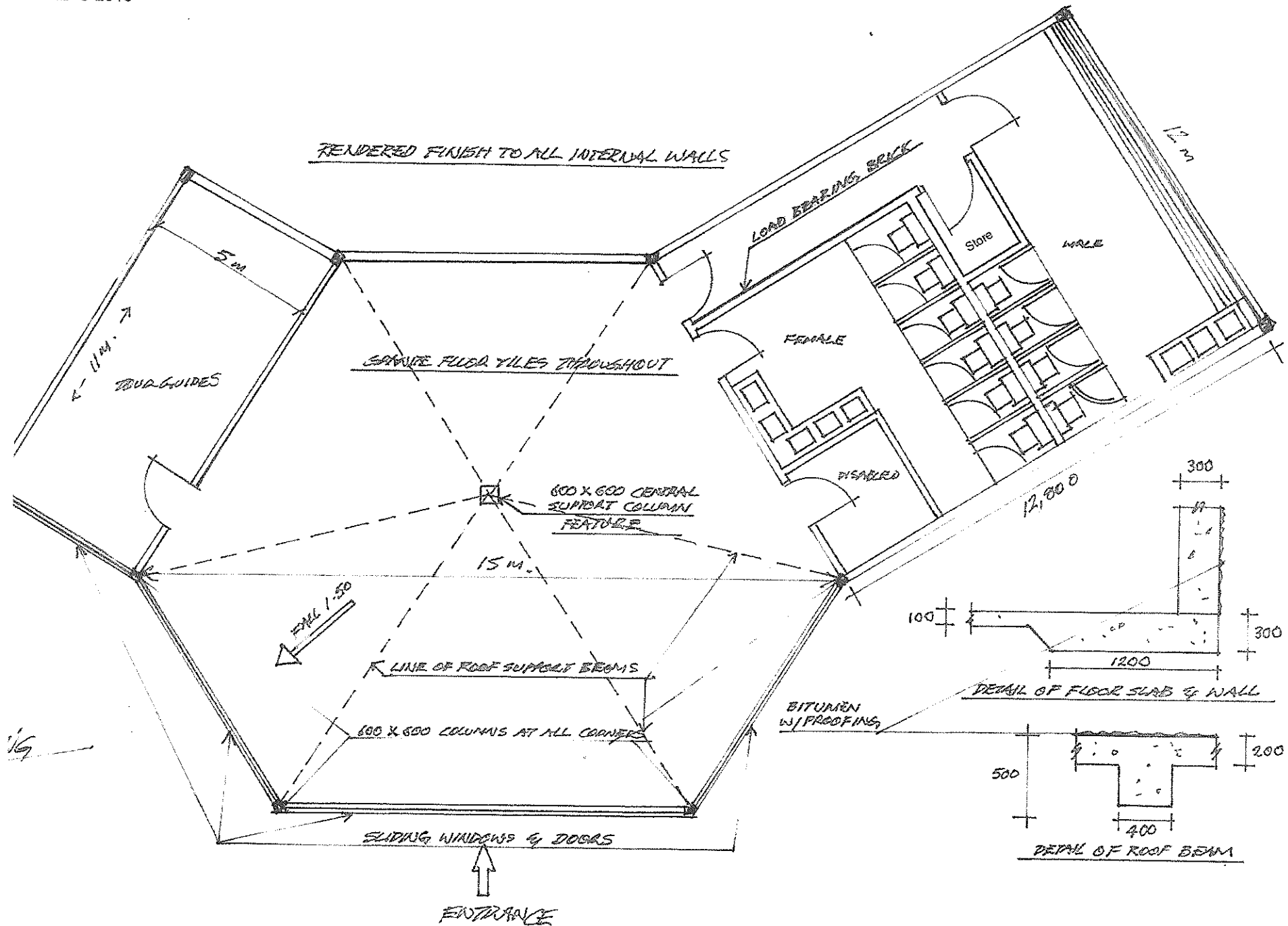
HMAS SYDNEY II BRIDGE - Rest & Amenities Area - PLAN
