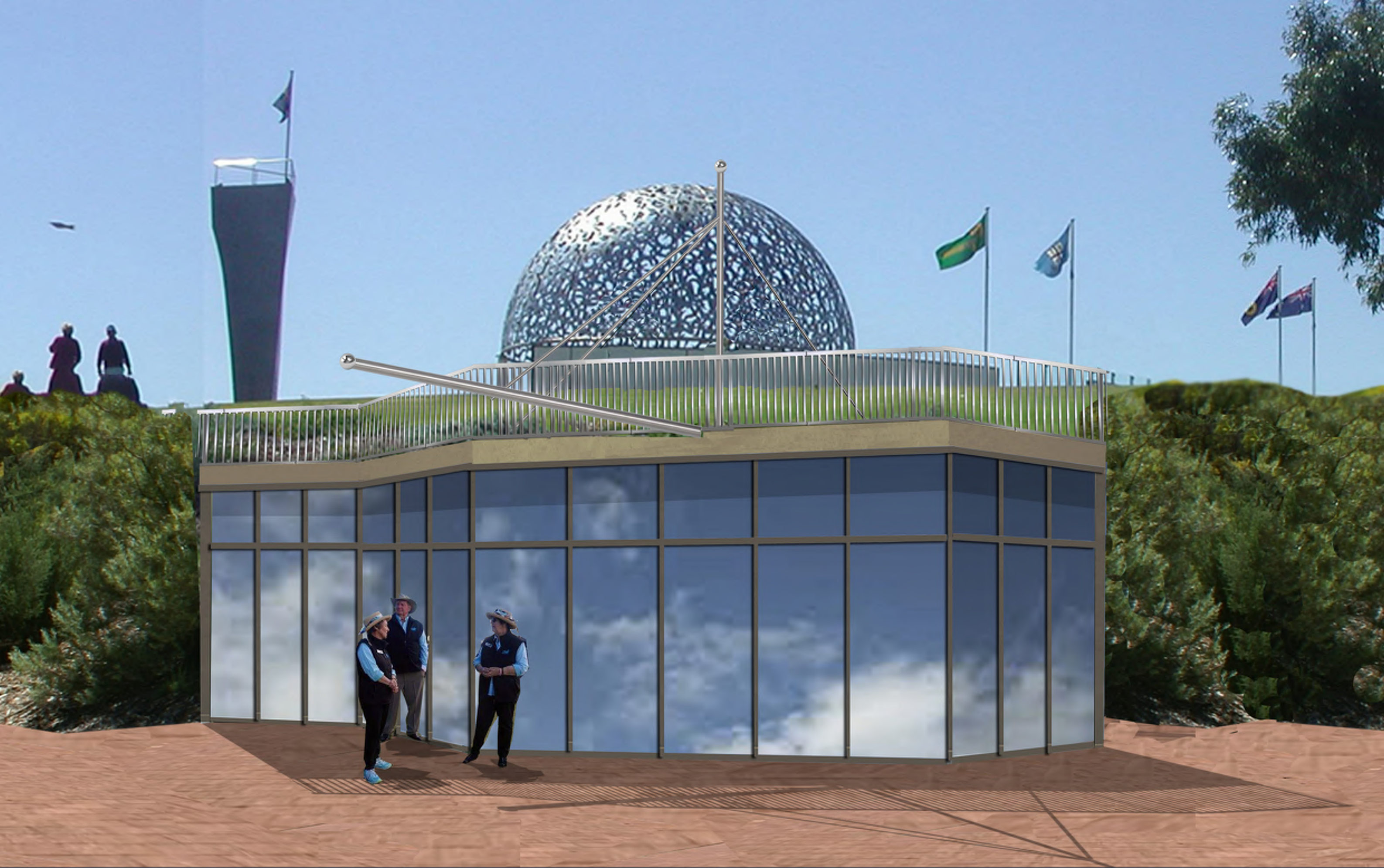
HMAS SYDNEY MEMORIAL GERALDTON WA OPTION 3A Elevation Visitor Guide Facility / HMAS Sydney II 'Bridge' Communal Space Built Into Hill
