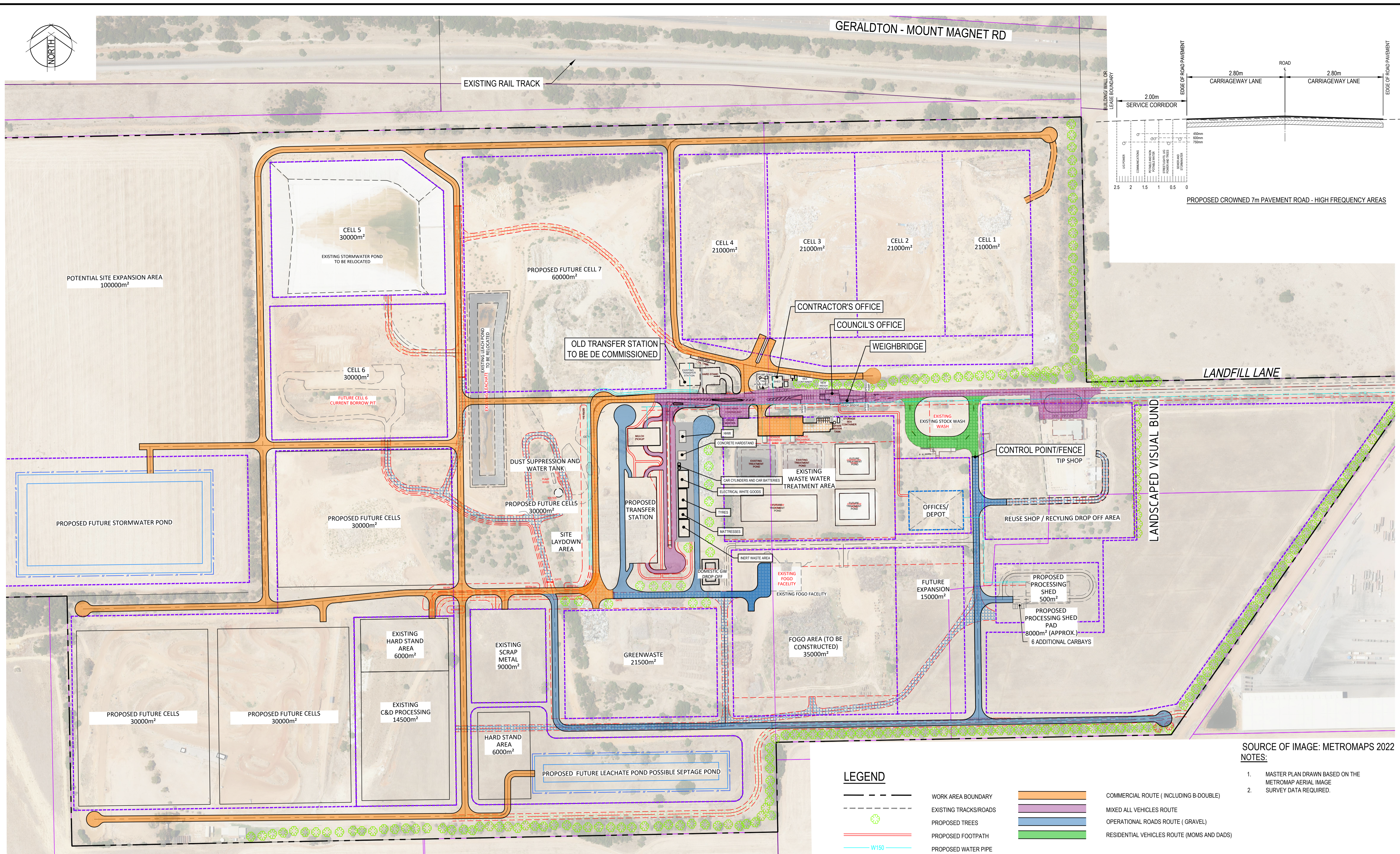
MERU WASTE FACILITY MASTER PLAN SCALE 1:2000
