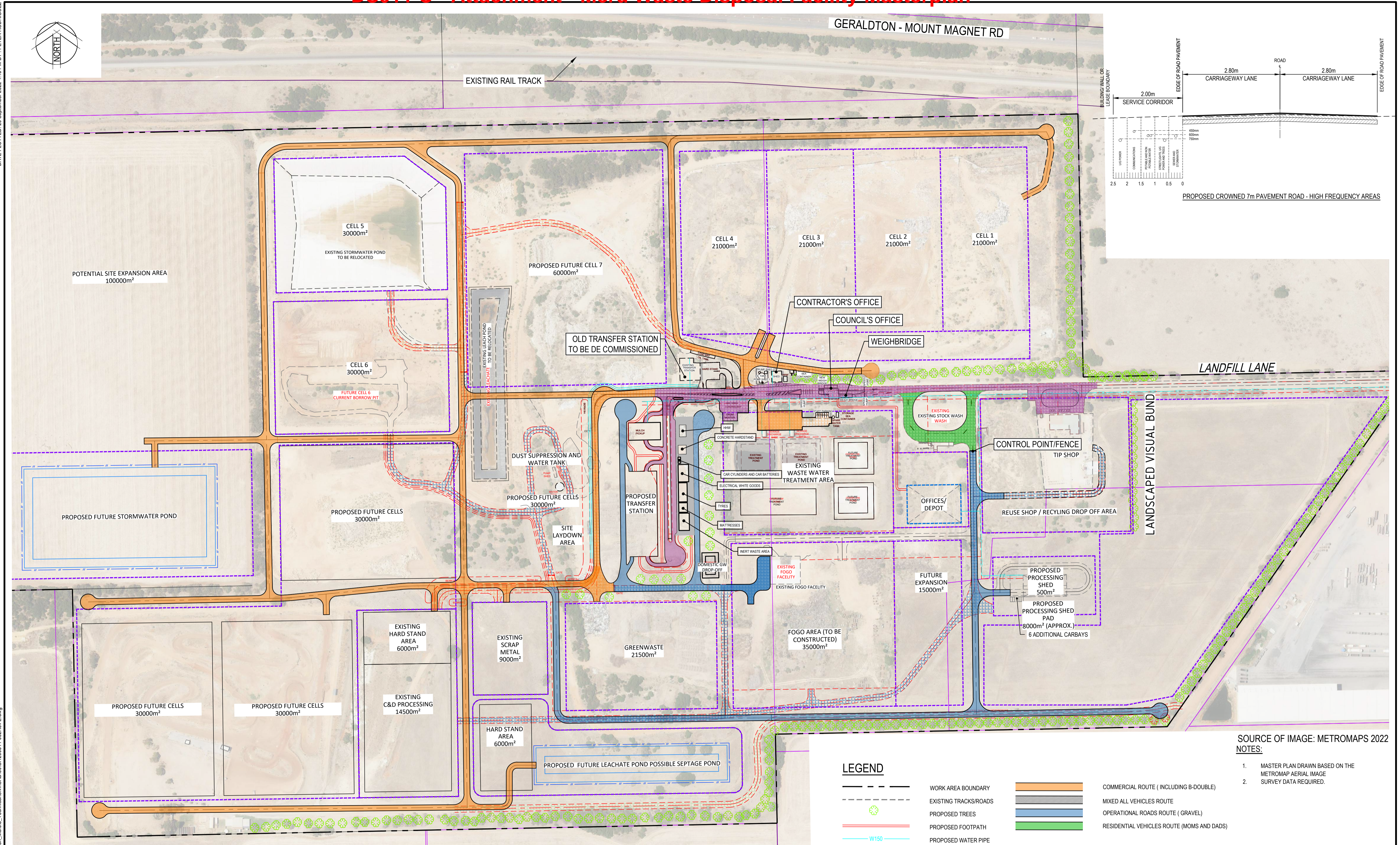
MERU WASTE FACILITY MASTER PLAN SCALE 1:2000
